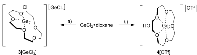
Scheme 2. a) \frac{1}{2} [15]crown-5; b) [15]crown-5, 2 \text{Me}_3\text{SiOTf} , -2 \text{Me}_3\text{SiCl} .
