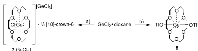
Scheme 3. a) 1.5 [18]crown-6; b) [18]crown-6, 2 \text{Me}_3\text{SiOTf} , -2 \text{Me}_3\text{SiCl} .
